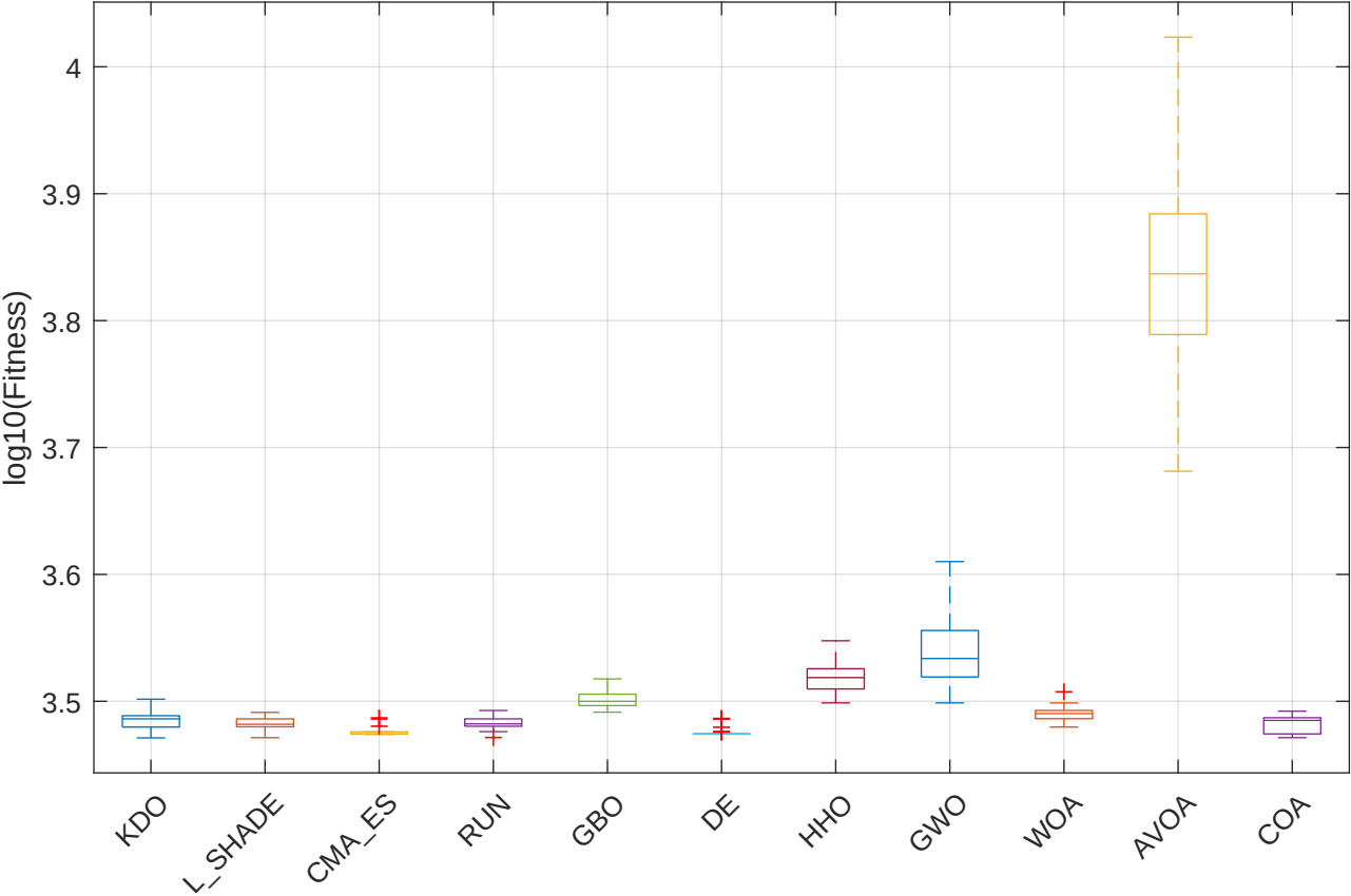
CEC2017 F25 (Numerical) - Boxplot
